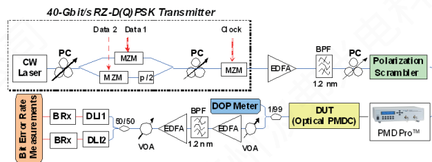
Figure 5. Experimental setup for PMD compensator performance test, using PMDPro™ as a PMD source to add DGD and SOPMD to the signal.
